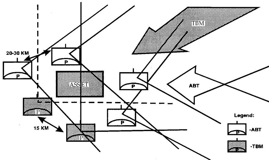
Figure 5-12. ABT-heavy defense.
