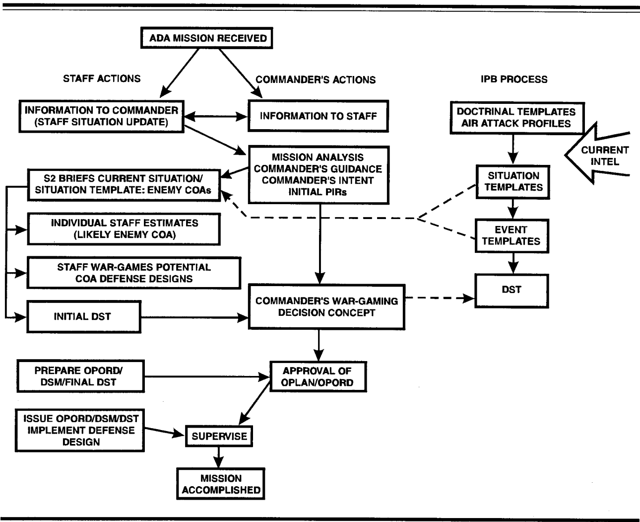
Figure 3-1. Decision process.
