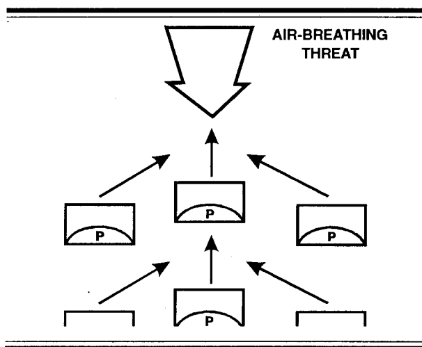
Figure 5-3. Convergent PTLs.
